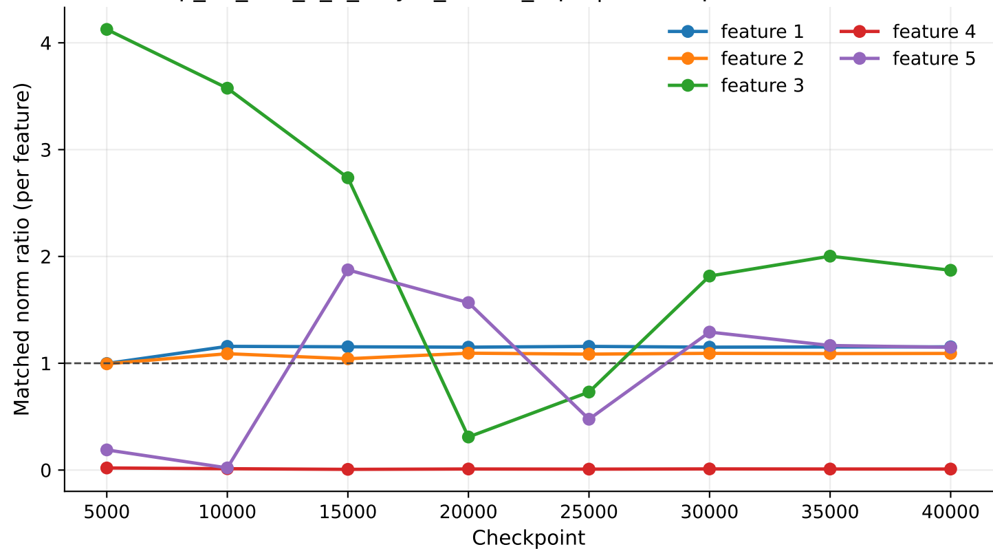
exp_07_tms_5_2_5layer_untied_rep1 | linear1 per-feature ML2R
