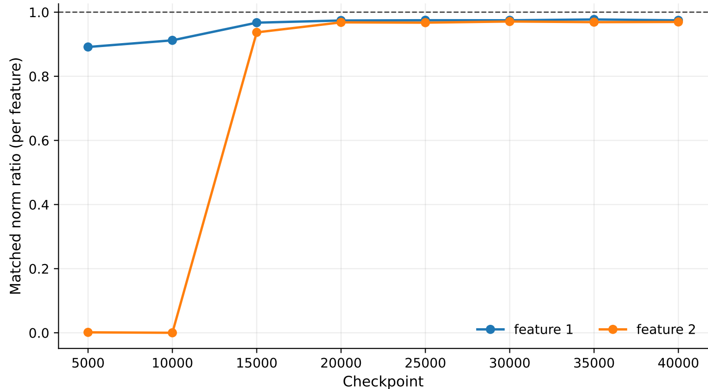
exp_07_tms_5_2_6layer_tied_rep1 | hidden_layers.0 per-feature ML2R
