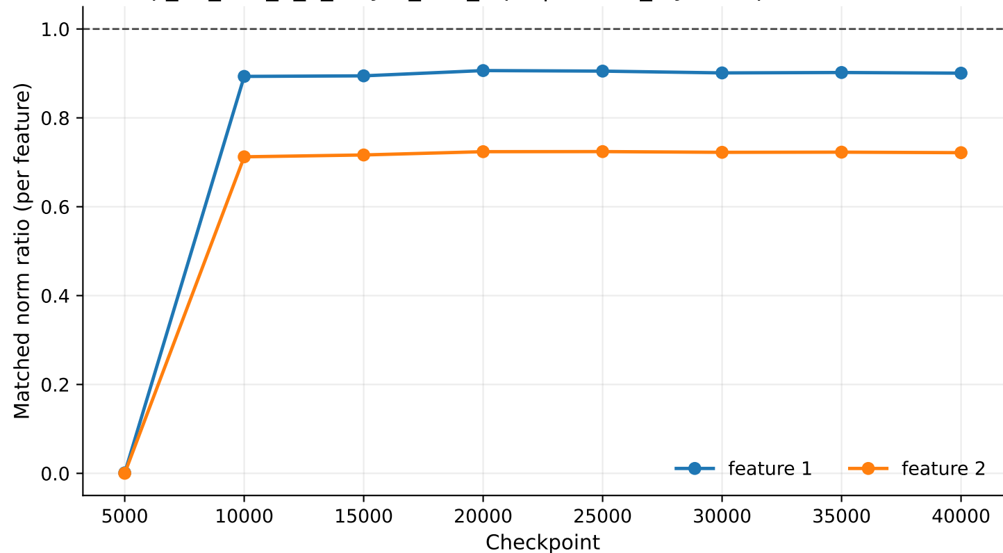
exp_07_tms_5_2_6layer_tied_rep1 | hidden_layers.1 per-feature ML2R
