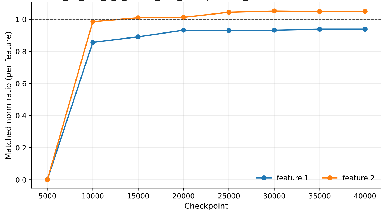
exp_07_tms_5_2_6layer_tied_rep1 | hidden_layers.3 per-feature ML2R
