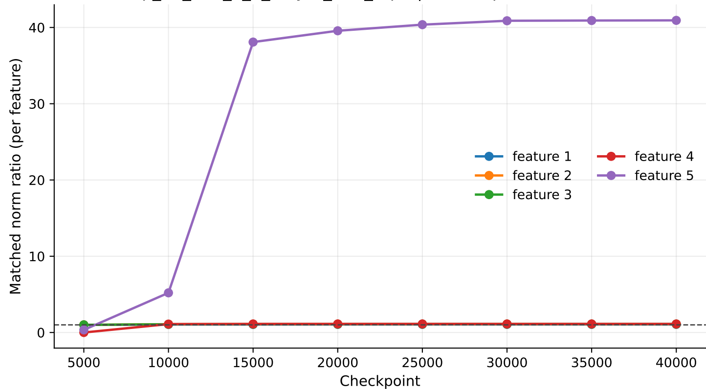
exp_07_tms_5_2_6layer_tied_rep1 | linear1 per-feature ML2R
