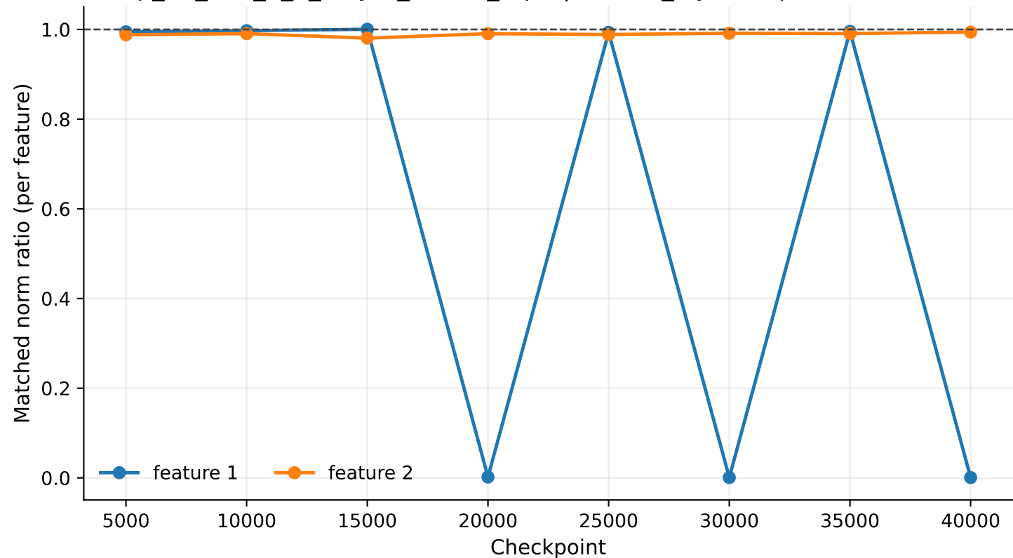
exp_07_tms_5_2_6layer_untied_rep1 | hidden_layers.0 per-feature ML2R
