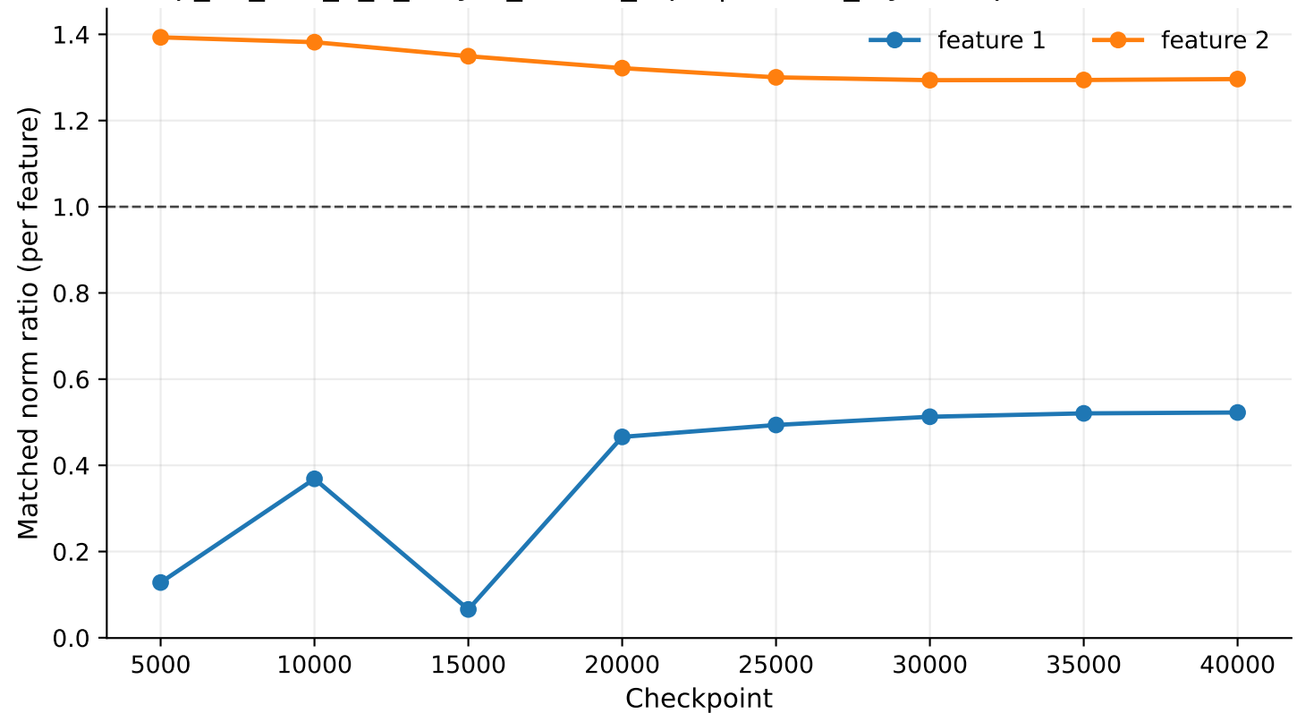
exp_07_tms_5_2_6layer_untied_rep1 | hidden_layers.2 per-feature ML2R
