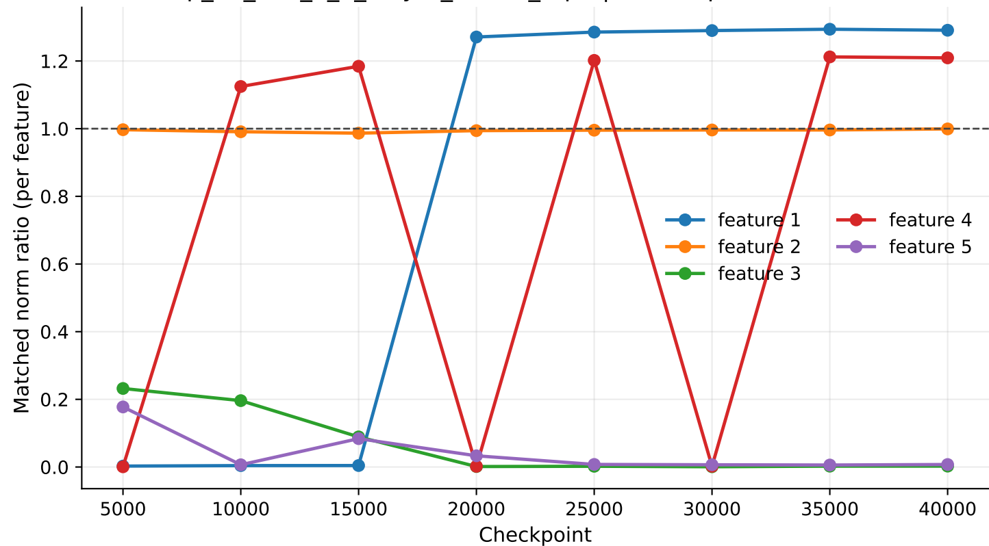
exp_07_tms_5_2_6layer_untied_rep1 | linear1 per-feature ML2R
