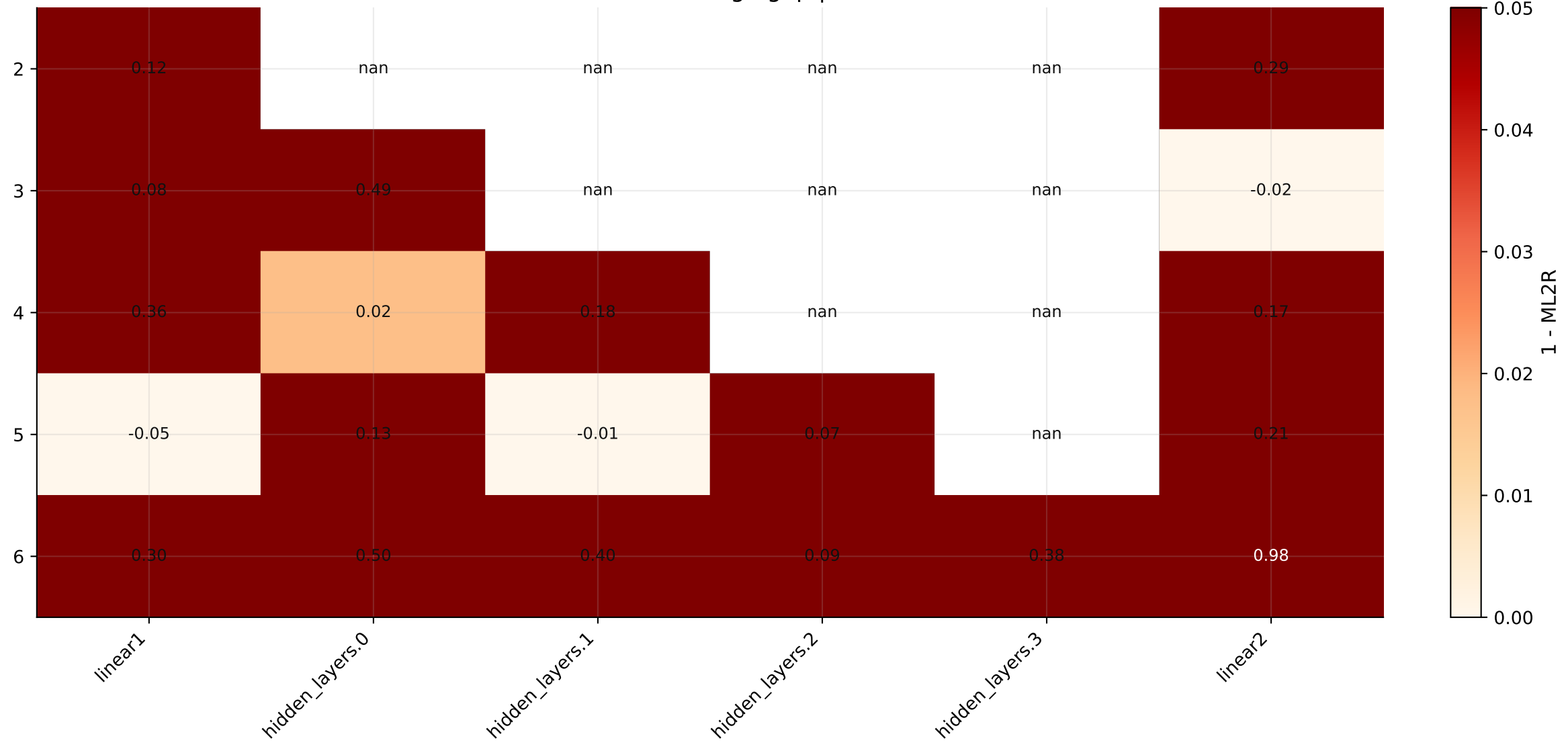
Final ML2R shrinkage gap | untied
