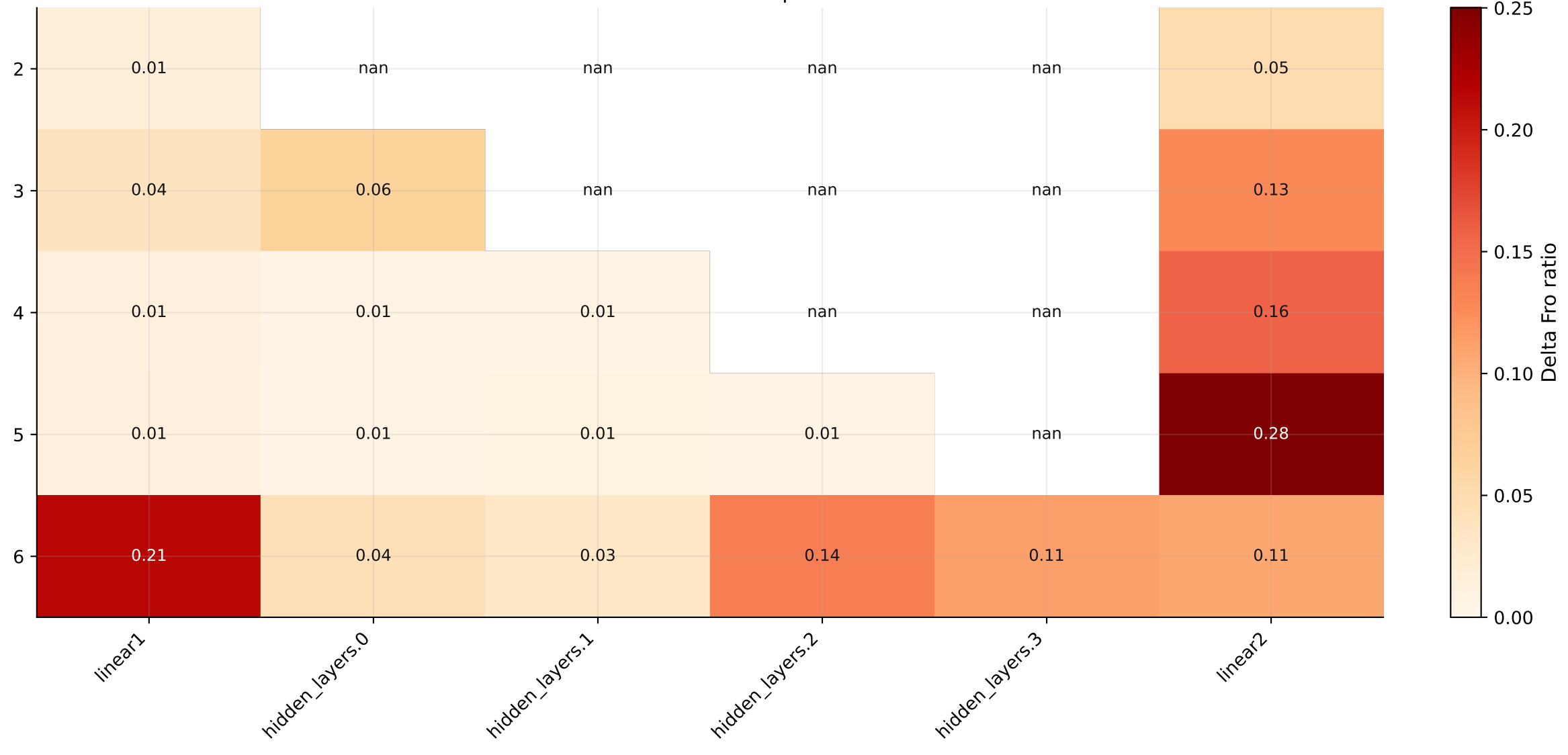
Final delta Fro ratio | untied
