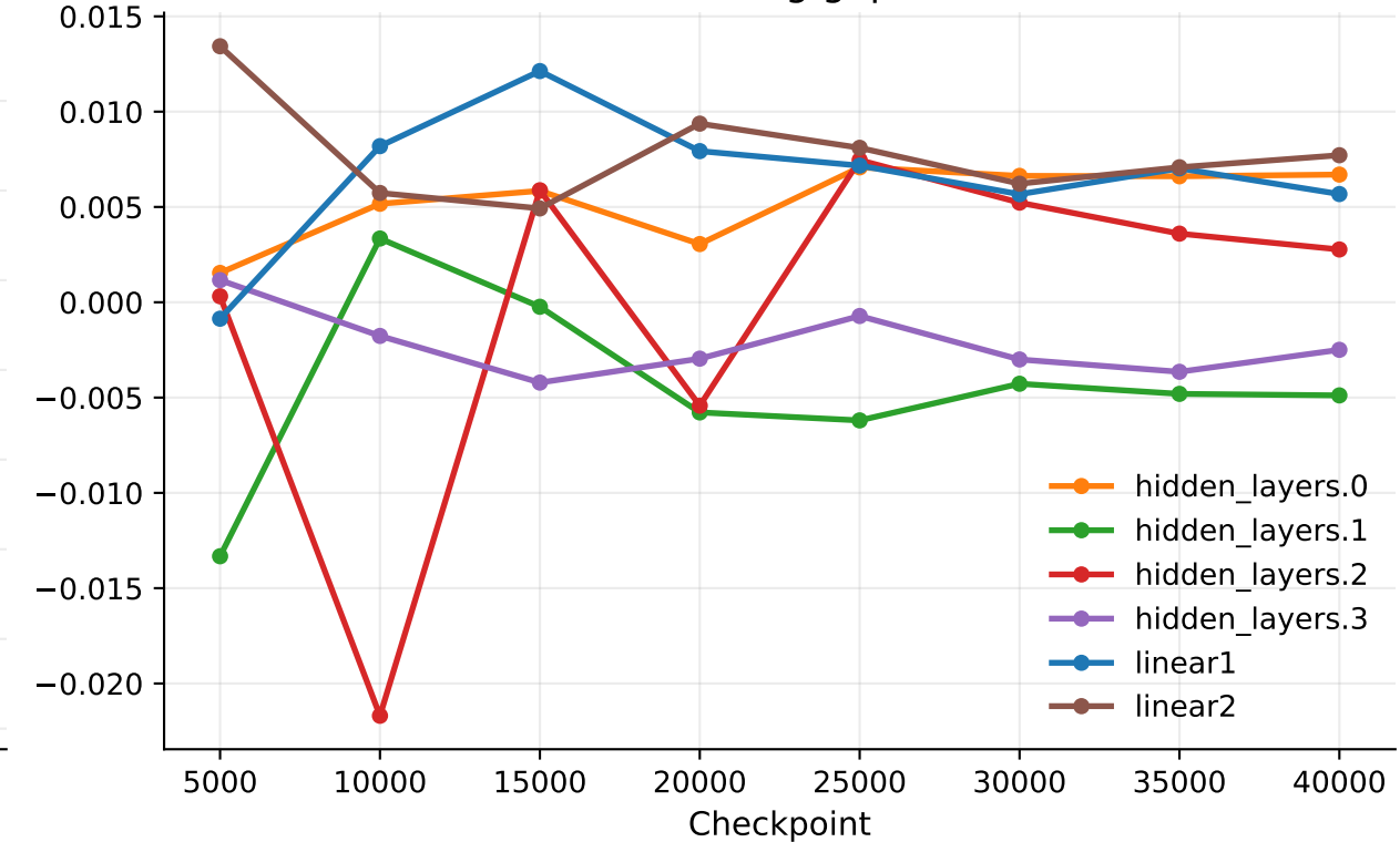
Raw under-scaling gap = 1 - ratio
