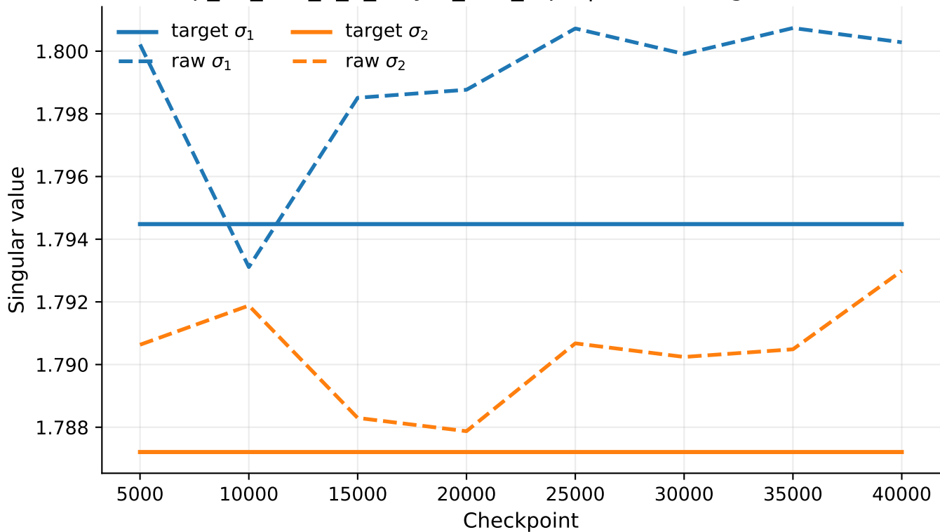
exp_07_tms_5_2_2layer_tied_rep1 | linear2 singular values
