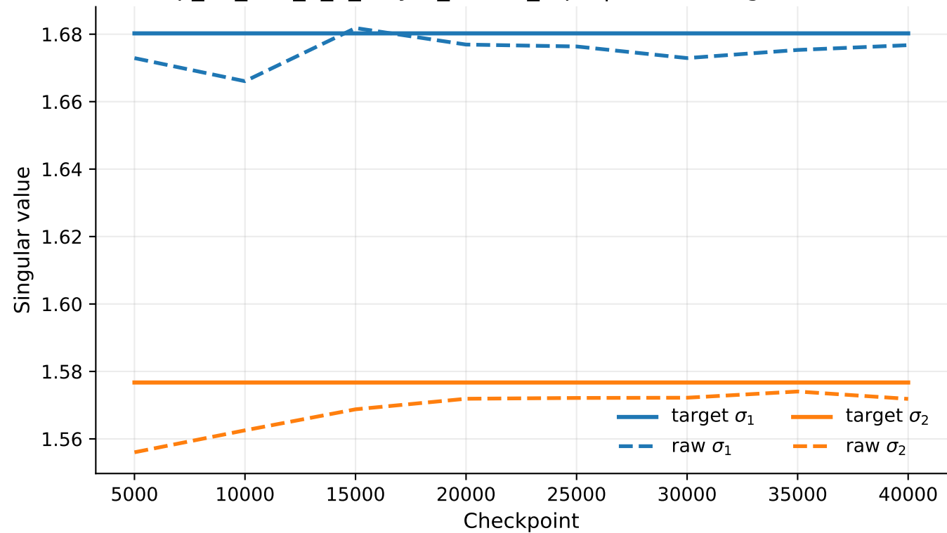
exp_07_tms_5_2_2layer_untied_rep1 | linear1 singular values
