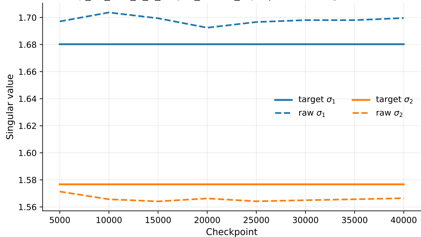
exp_07_tms_5_2_2layer_untied_rep1 | linear2 singular values
