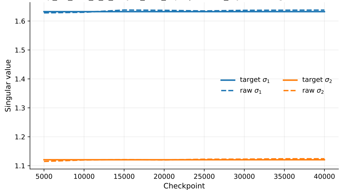
exp_07_tms_5_2_3layer_tied_rep1 | hidden_layers.0 singular values
