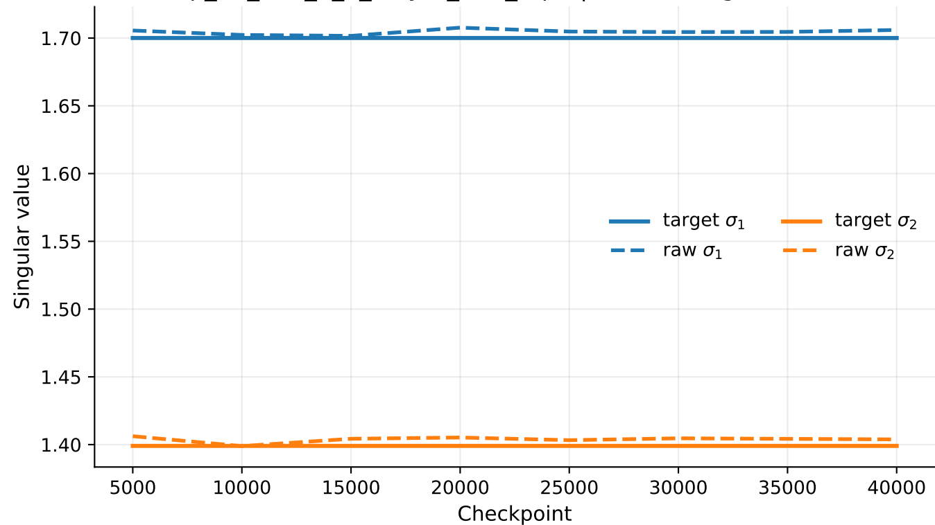
exp_07_tms_5_2_3layer_tied_rep1 | linear1 singular values
