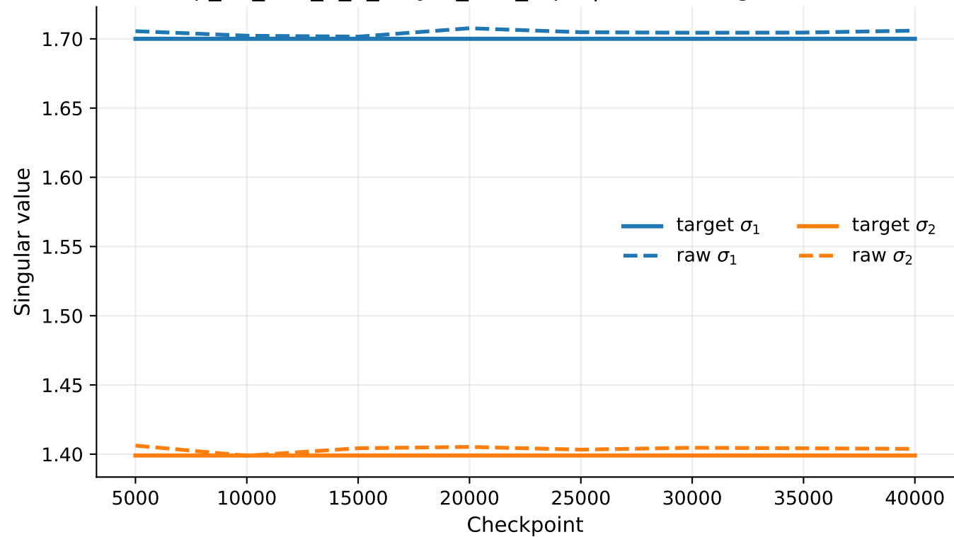
exp_07_tms_5_2_3layer_tied_rep1 | linear2 singular values
