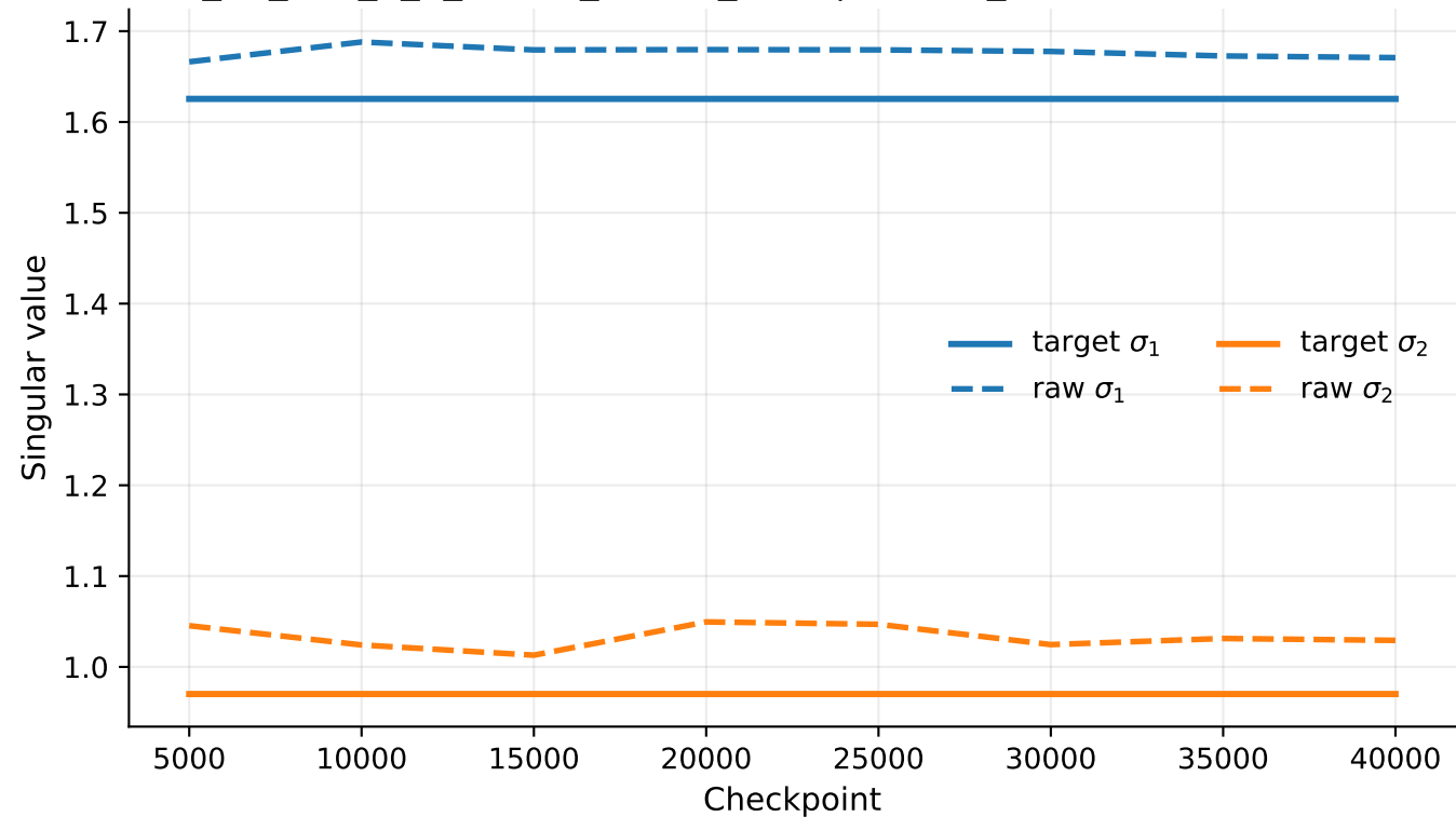
exp_07_tms_5_2_3layer_untied_rep1 | hidden_layers.0 singular values
