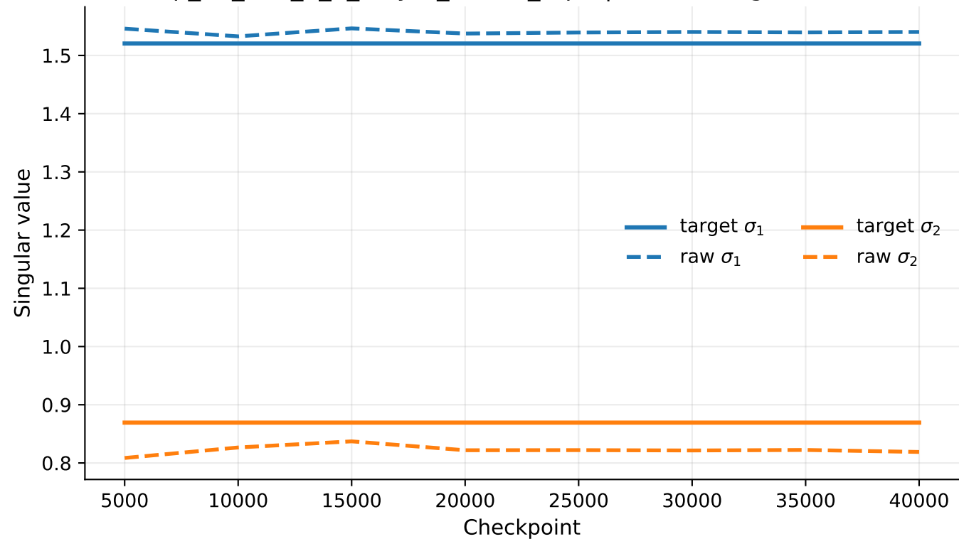
exp_07_tms_5_2_3layer_untied_rep1 | linear1 singular values
