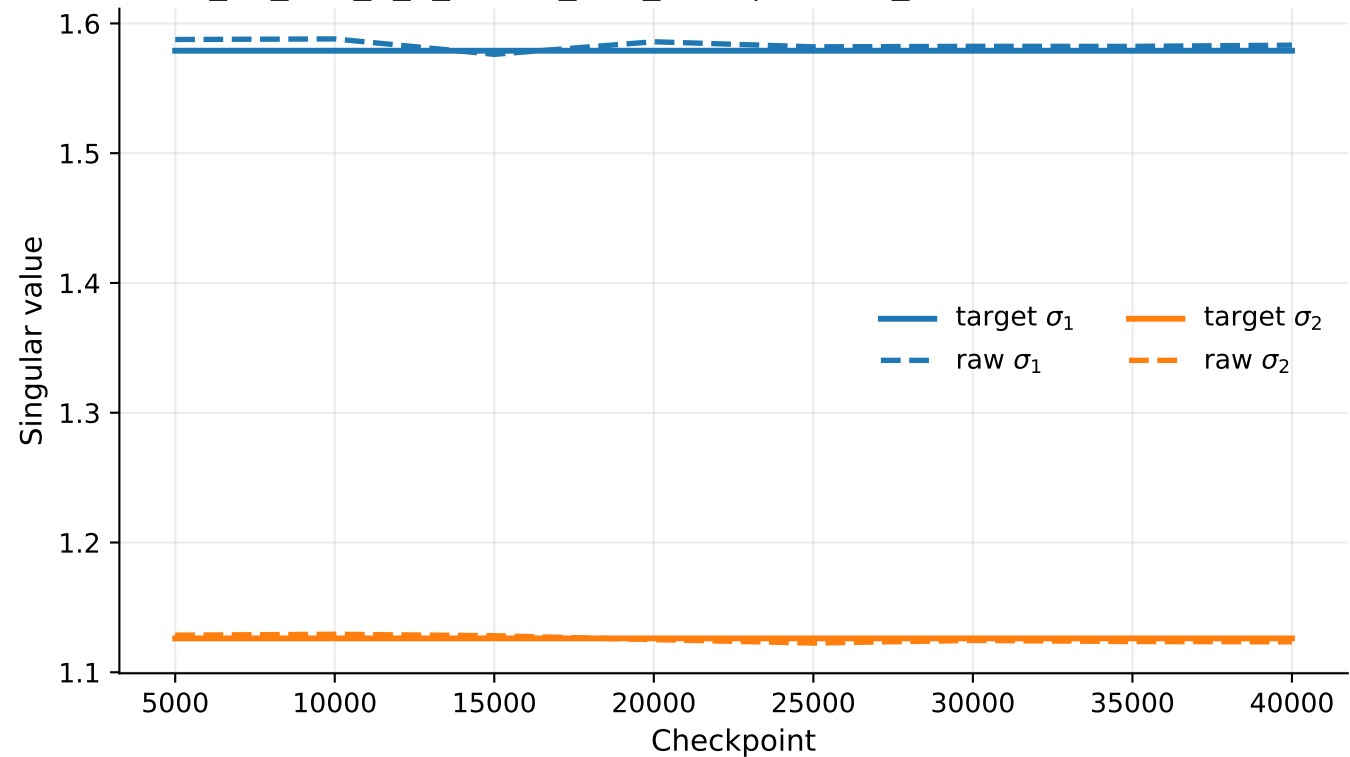
exp_07_tms_5_2_4layer_tied_rep1 | hidden_layers.0 singular values
