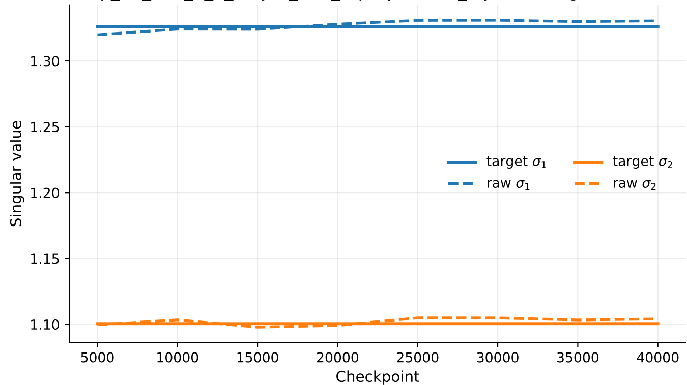
exp_07_tms_5_2_4layer_tied_rep1 | hidden_layers.1 singular values
