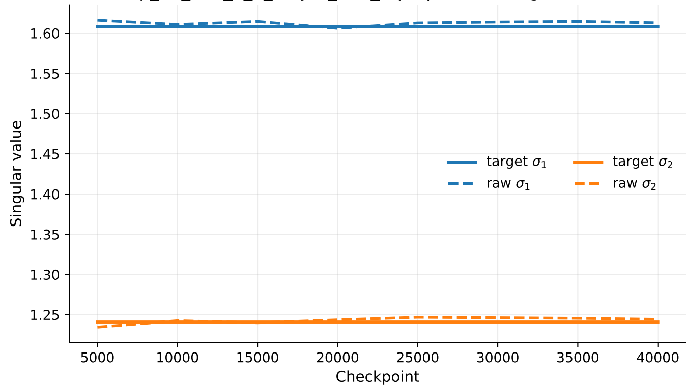
exp_07_tms_5_2_4layer_tied_rep1 | linear1 singular values
