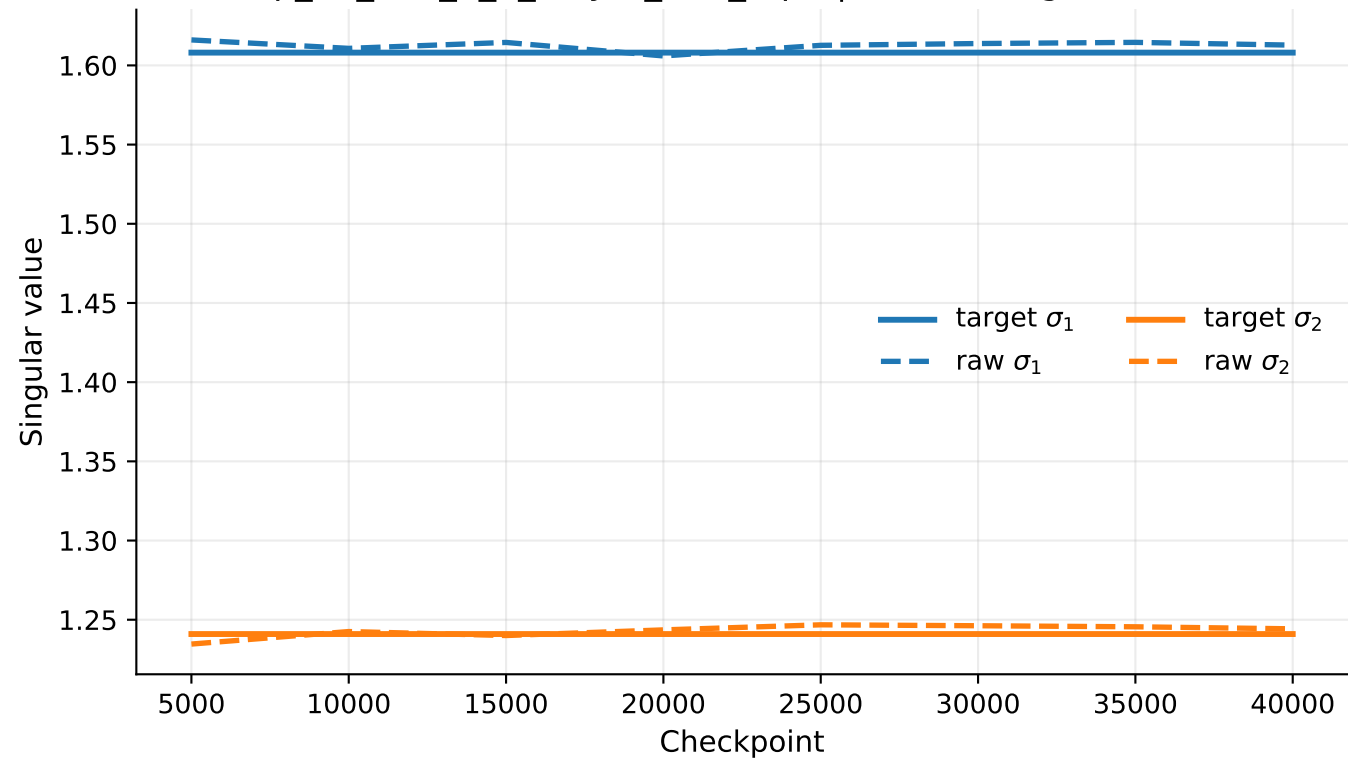
exp_07_tms_5_2_4layer_tied_rep1 | linear2 singular values
