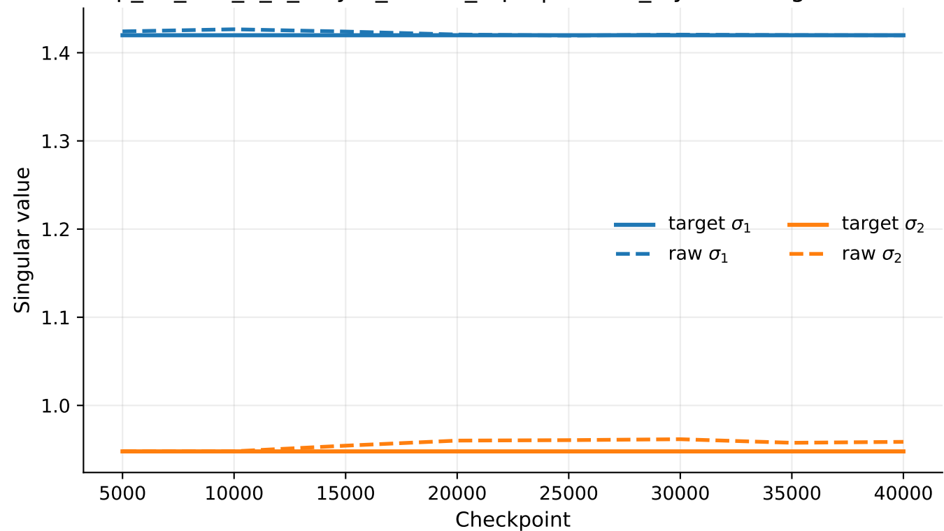
exp_07_tms_5_2_4layer_untied_rep1 | hidden_layers.1 singular values
