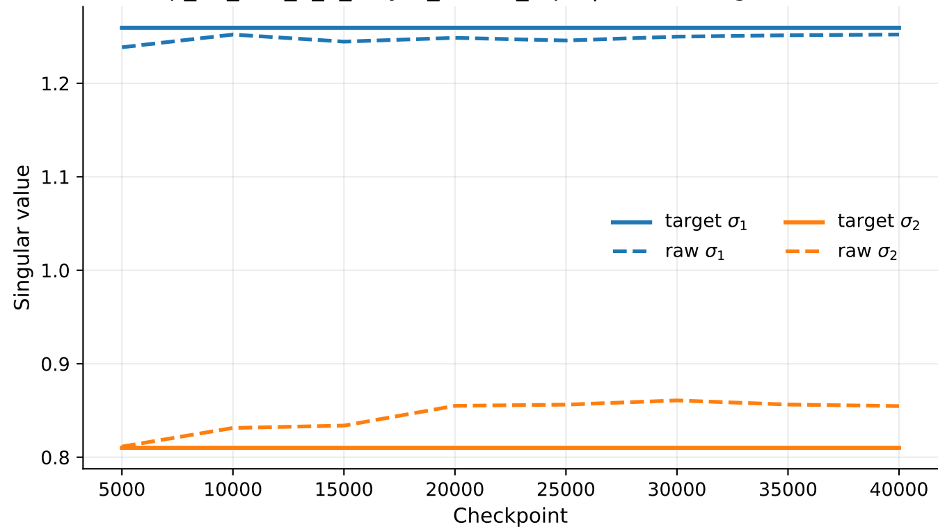
exp_07_tms_5_2_4layer_untied_rep1 | linear2 singular values
