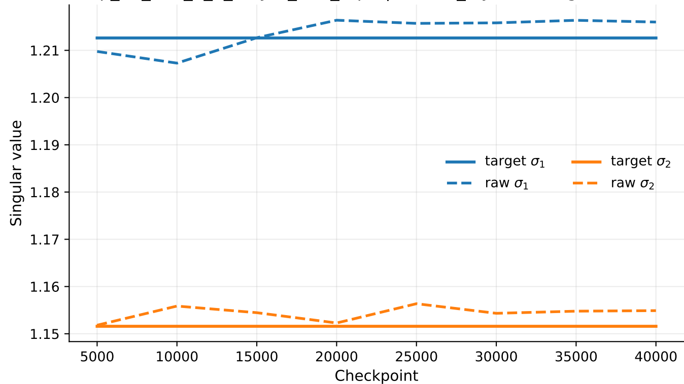
exp_07_tms_5_2_5layer_tied_rep1 | hidden_layers.1 singular values
