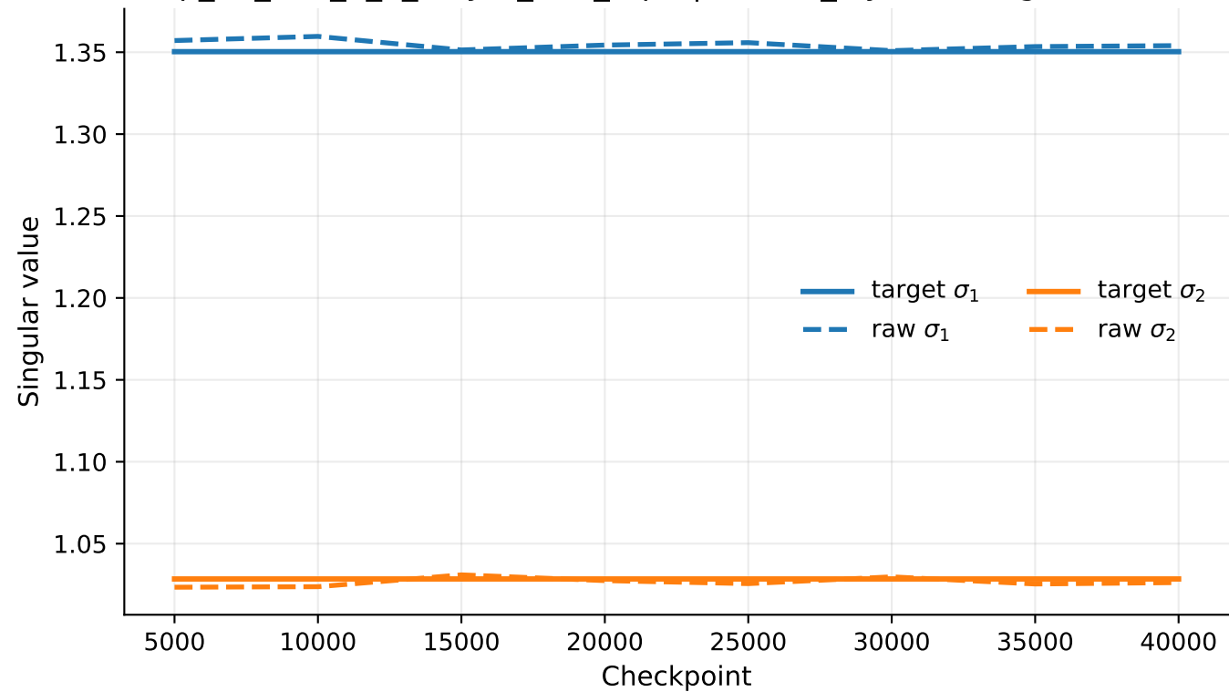
exp_07_tms_5_2_5layer_tied_rep1 | hidden_layers.2 singular values
