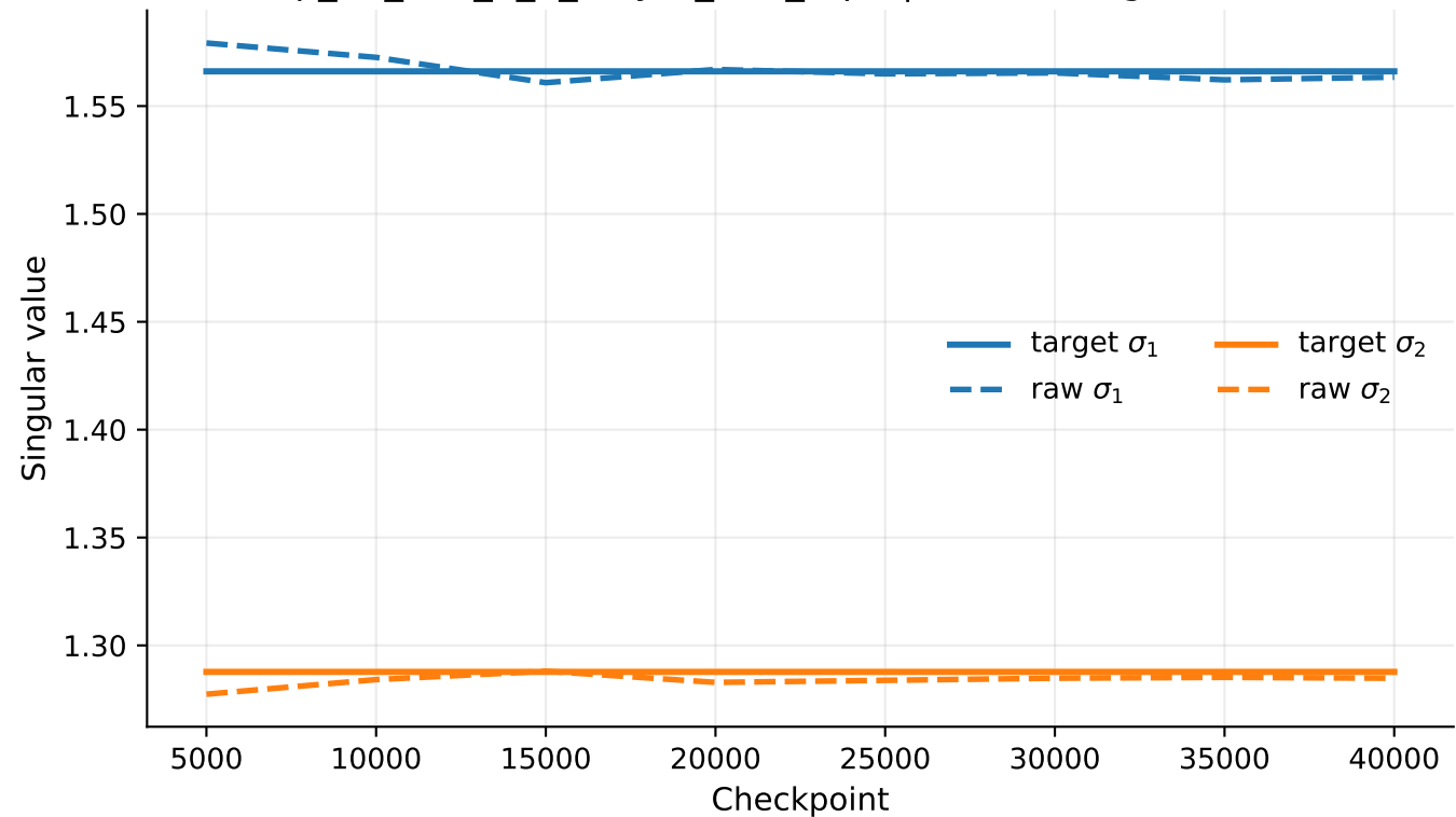
exp_07_tms_5_2_5layer_tied_rep1 | linear1 singular values
