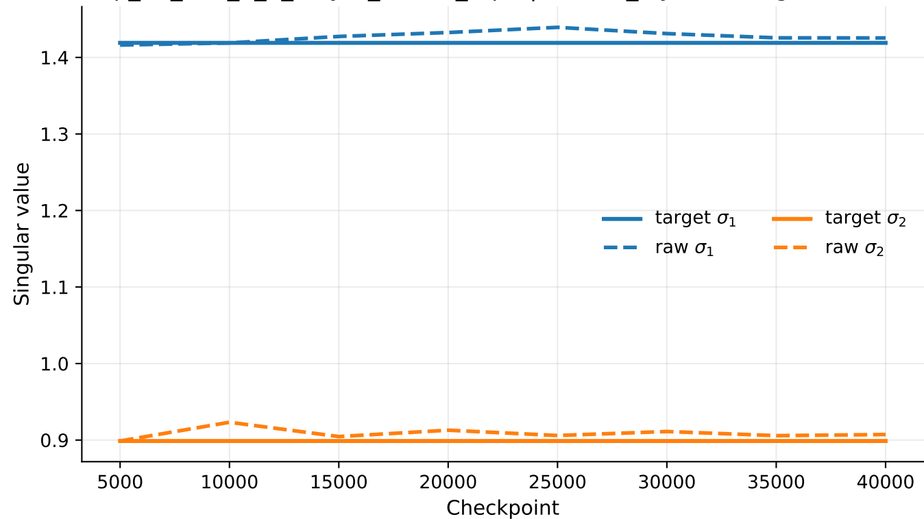
exp_07_tms_5_2_5layer_untied_rep1 | hidden_layers.0 singular values
