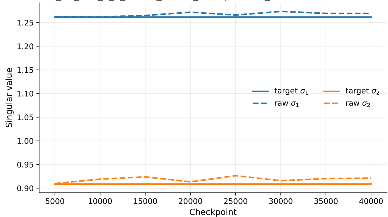
exp_07_tms_5_2_5layer_untied_rep1 | hidden_layers.1 singular values
