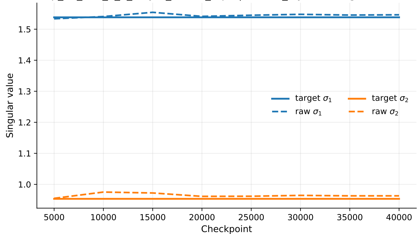
exp_07_tms_5_2_5layer_untied_rep1 | hidden_layers.2 singular values
