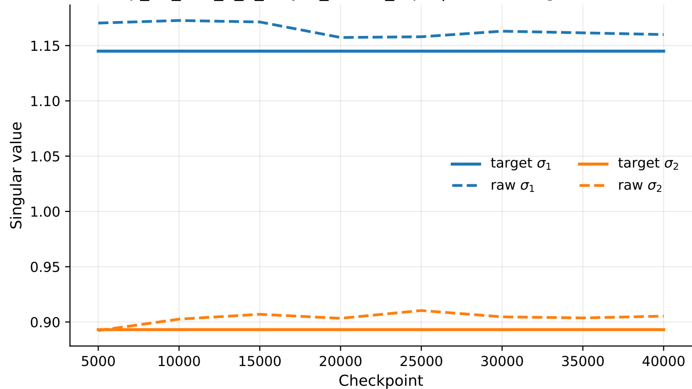
exp_07_tms_5_2_5layer_untied_rep1 | linear1 singular values
