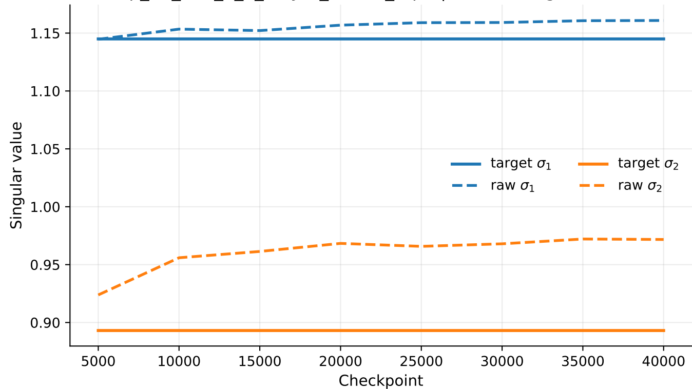
exp_07_tms_5_2_5layer_untied_rep1 | linear2 singular values
