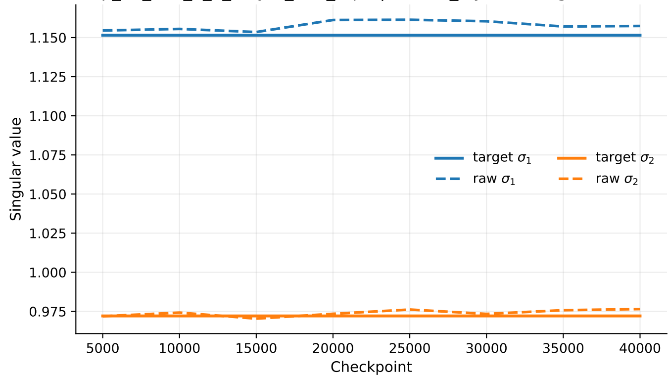
exp_07_tms_5_2_6layer_tied_rep1 | hidden_layers.0 singular values
