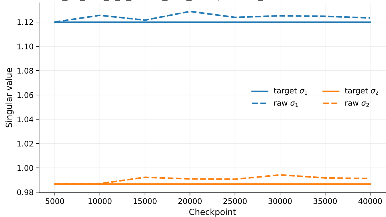
exp_07_tms_5_2_6layer_tied_rep1 | hidden_layers.1 singular values
