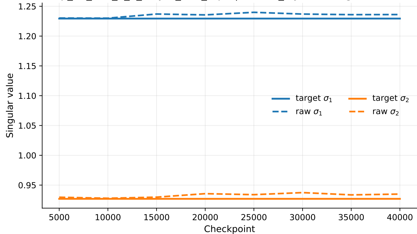
exp_07_tms_5_2_6layer_tied_rep1 | hidden_layers.3 singular values
