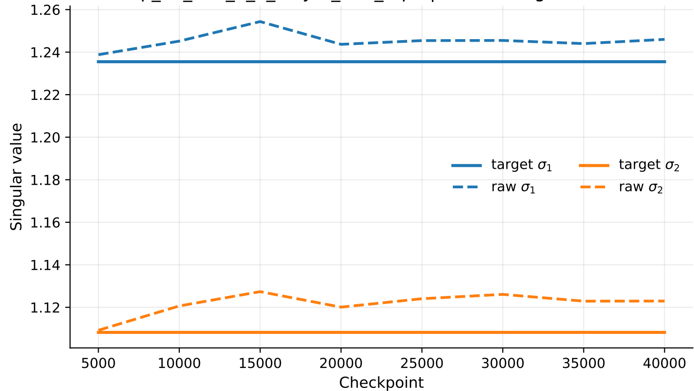
exp_07_tms_5_2_6layer_tied_rep1 | linear1 singular values
