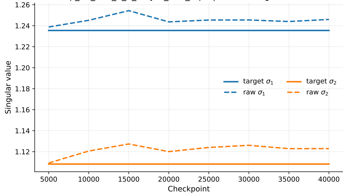
exp_07_tms_5_2_6layer_tied_rep1 | linear2 singular values
