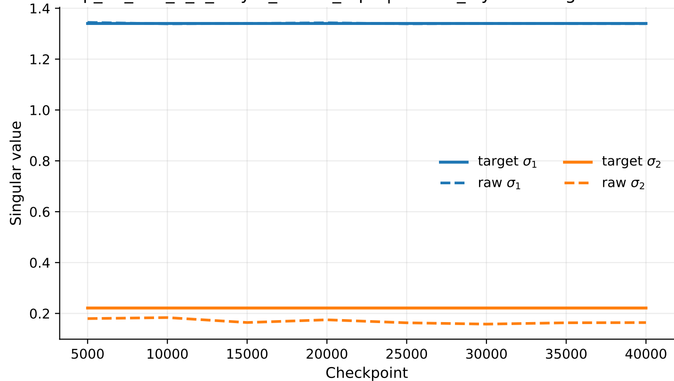
exp_07_tms_5_2_6layer_untied_rep1 | hidden_layers.0 singular values
