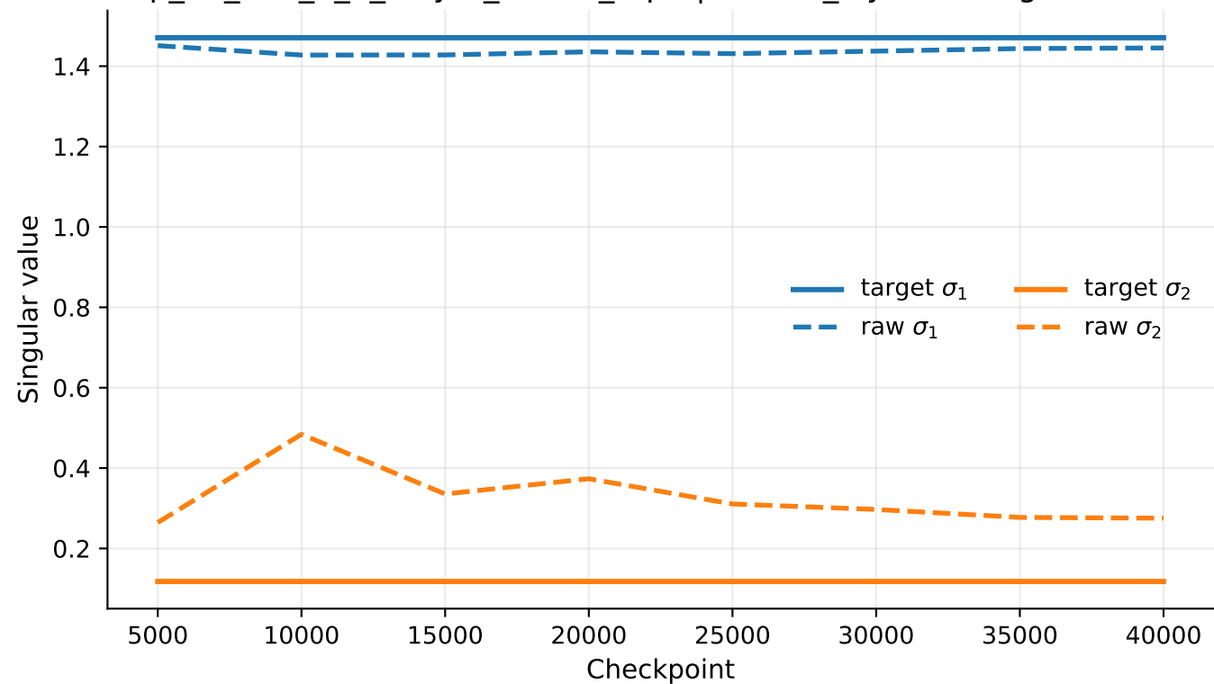
exp_07_tms_5_2_6layer_untied_rep1 | hidden_layers.2 singular values
