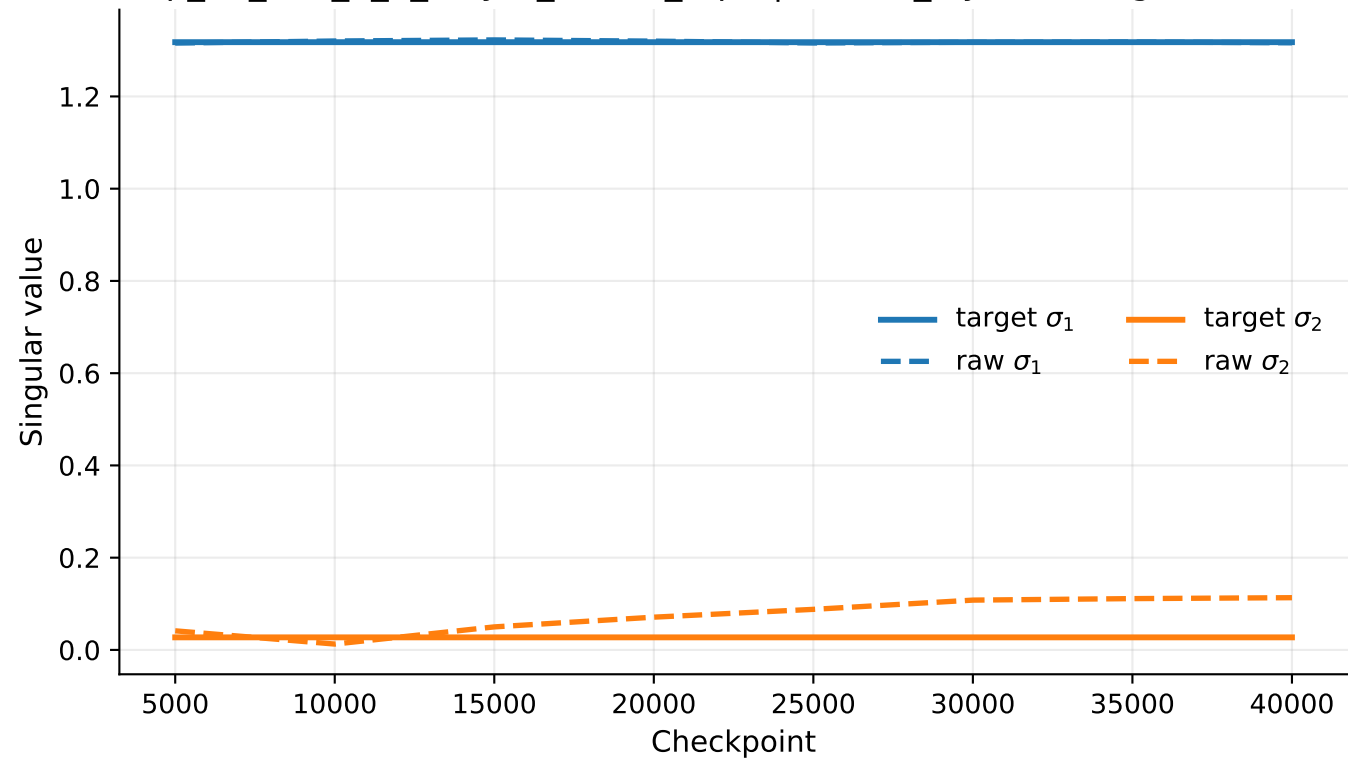
exp_07_tms_5_2_6layer_untied_rep1 | hidden_layers.3 singular values
