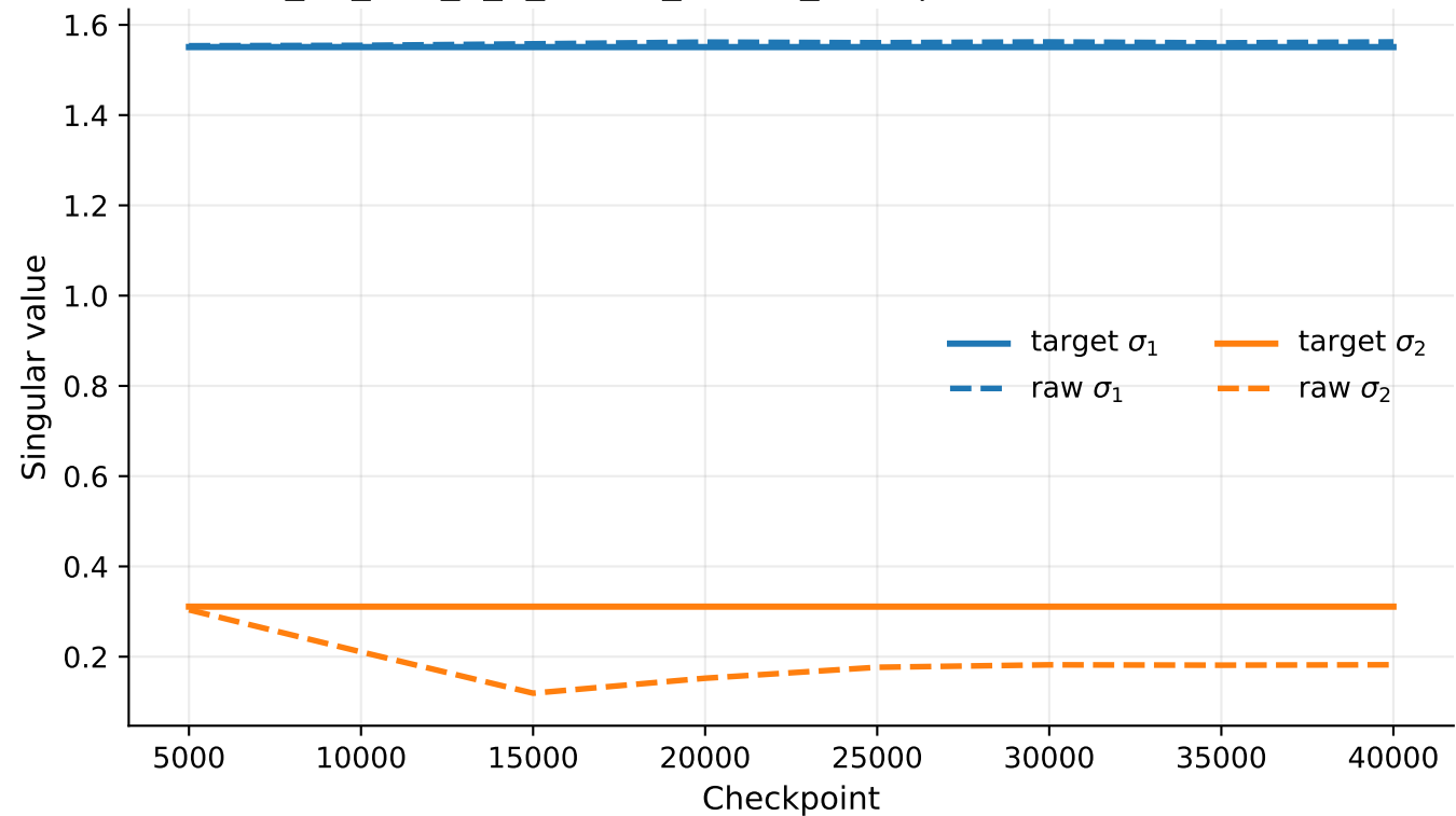
exp_07_tms_5_2_6layer_untied_rep1 | linear1 singular values
