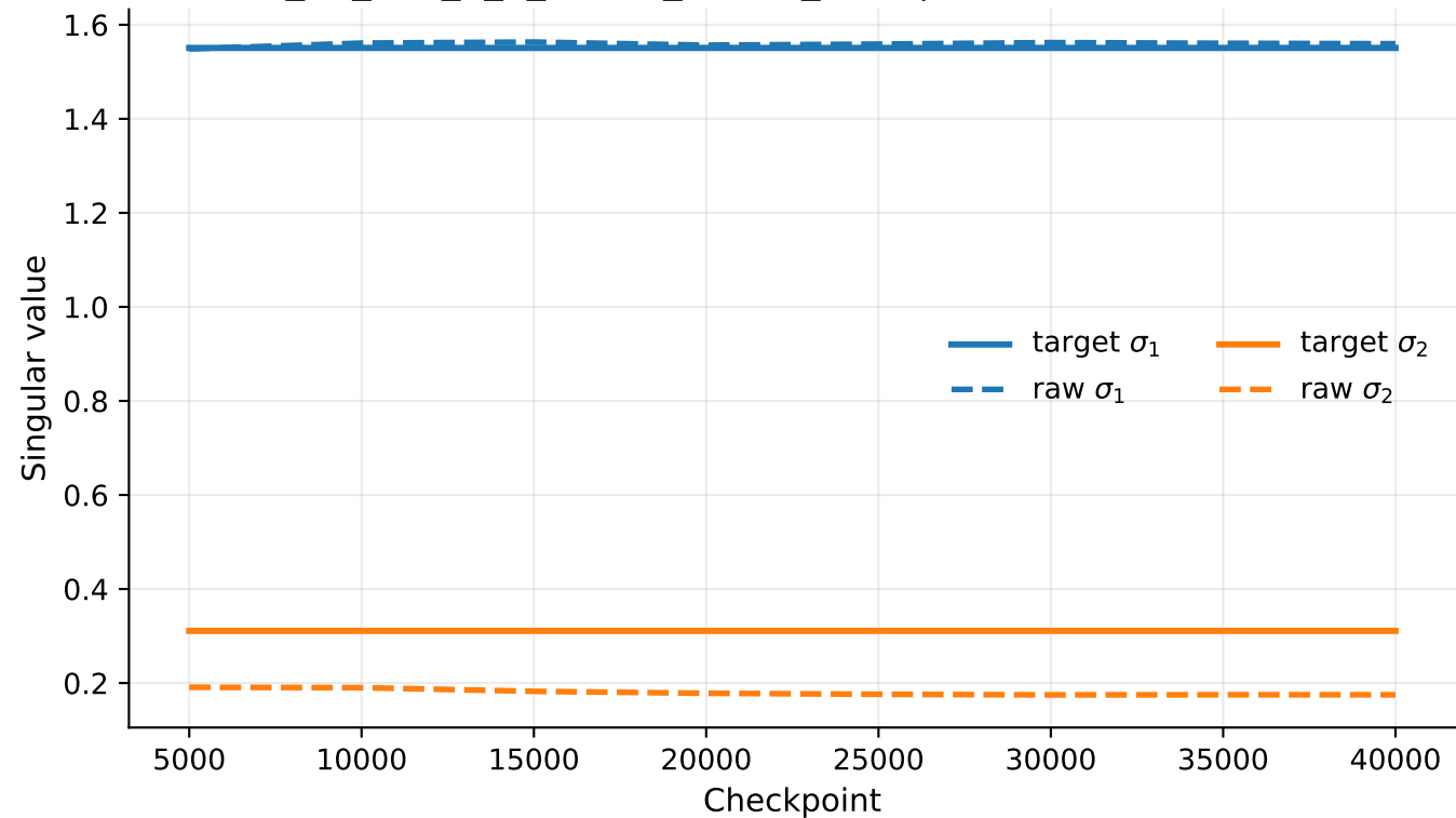
exp_07_tms_5_2_6layer_untied_rep1 | linear2 singular values
