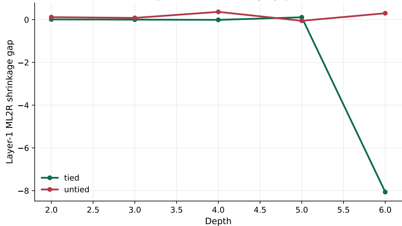
Layer-1 ML2R shrinkage gap
