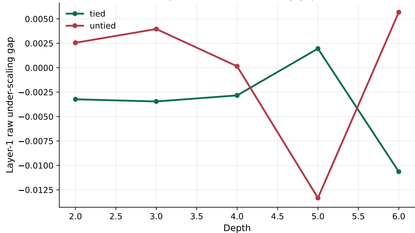
Layer-1 raw under-scaling gap
