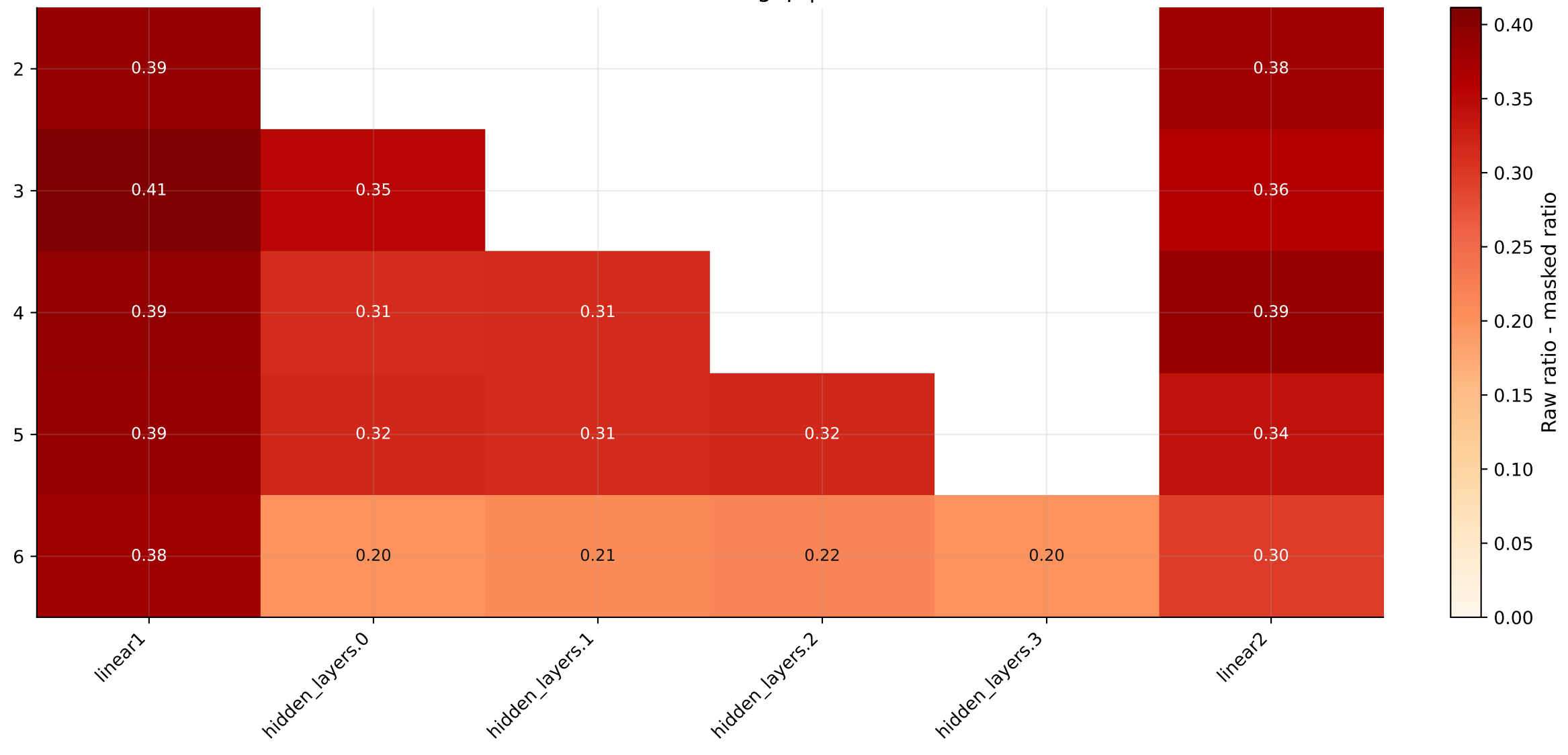
Final CI attenuation gap | untied
