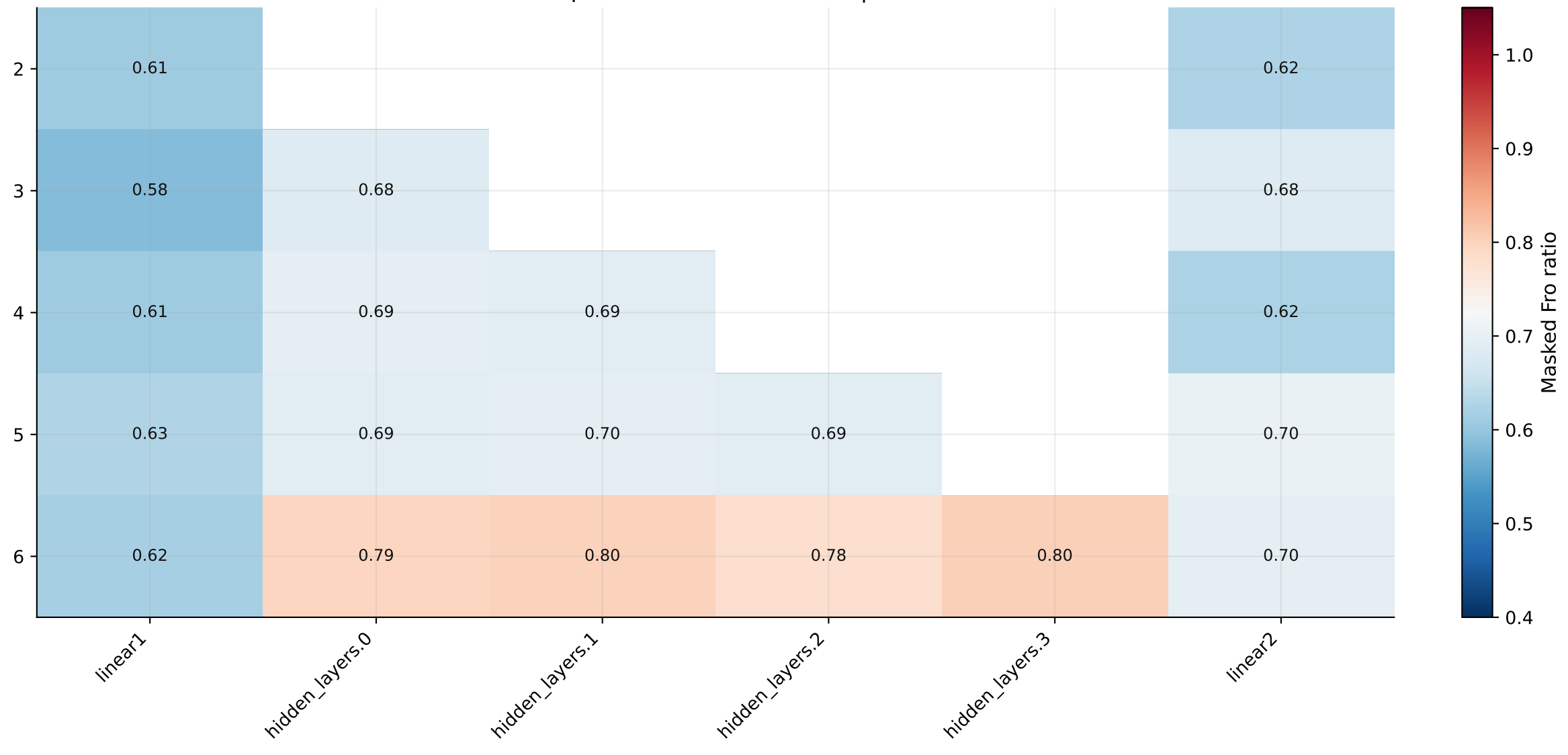
Final expected masked Fro ratio | untied
