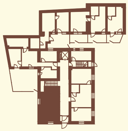
Plan parteru
