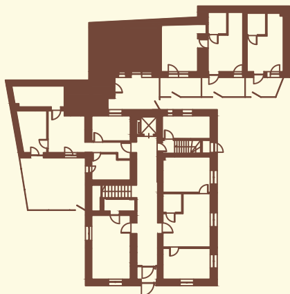
Plan parteru
