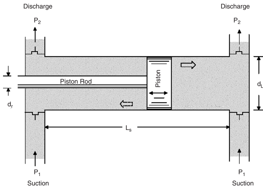
Figure 1.14 Double-action piston pump.
