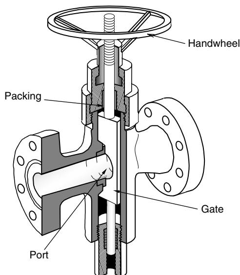
Figure 1.11 A sketch of a surface valve.
