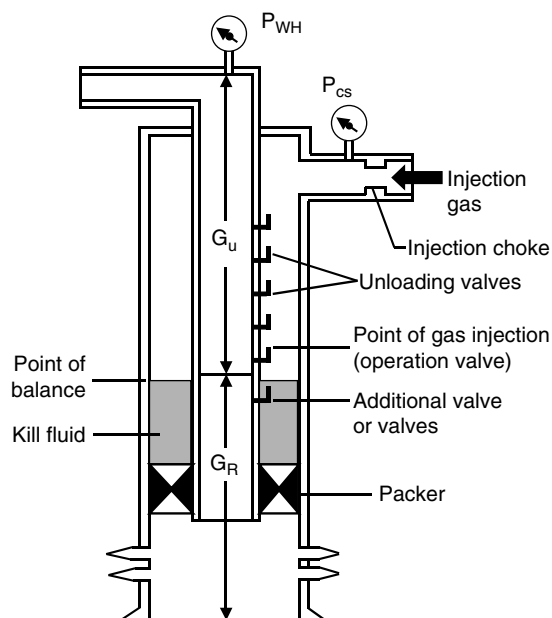
Figure 13.3 A sketch of continuous gas lift.
