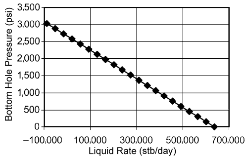
Figure 3.16 Composite IPR curve for all the layers open to flow.
