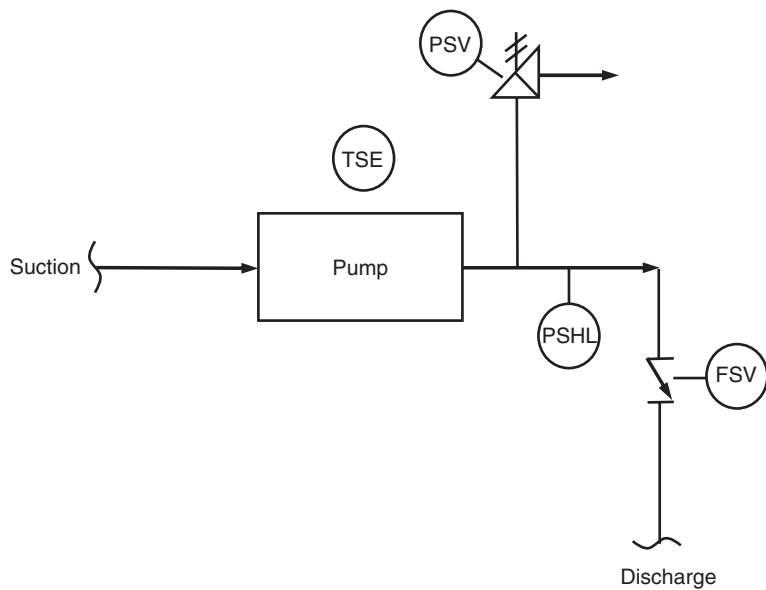
Figure 1.22 Safety system design for other pumps.
