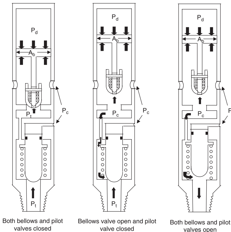
Figure 13.17 A sketch of combination valve.
