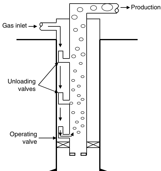
Figure 13.1 Configuration of a typical gas lift well.
