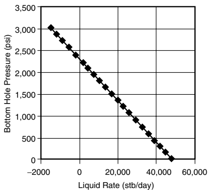
Figure 3.18 Composite IPR curve for Group 3 (Layers B1, A4, and A5).
