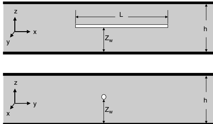
Figure 15.2 Notations for a horizontal wellbore.
