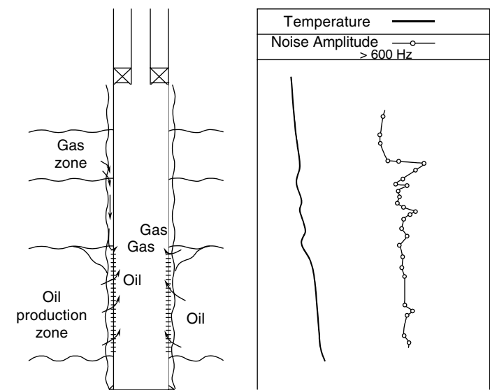
Figure 15.12 Temperature and noise logs identifying gas channeling behind casing (Economides et al., 1994).
