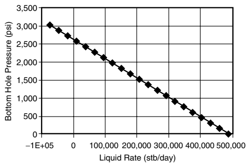
Figure 3.17 Composite IPR curve for Group 2 (Layers B4, C1, and C2).
