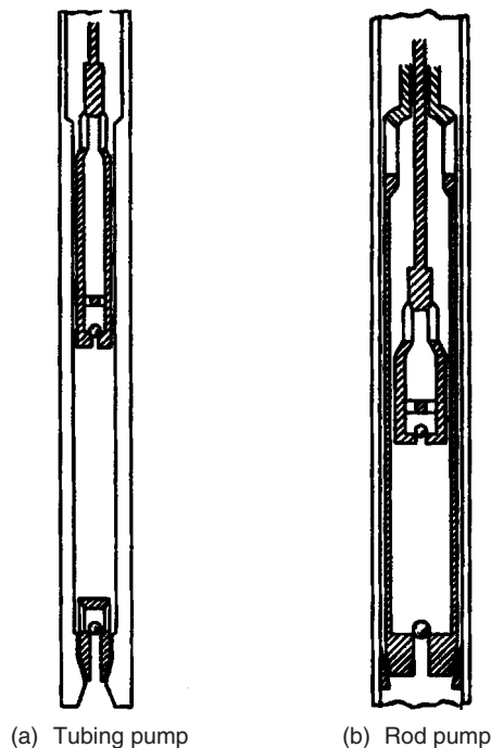
Figure 12.4 Two types of plunger pumps (Nind, 1964).
