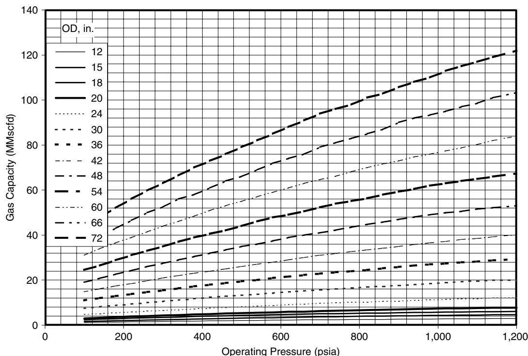
Figure 10.10 Gas capacity for trayed glycol contactors based on 0.7-specific gravity at 100 °F (Sivalis, 1977).
