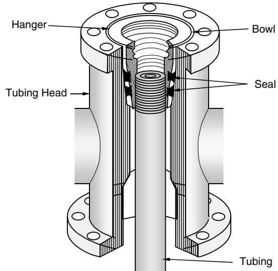
Figure 1.9 A sketch of a tubing head.
