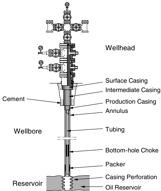
Figure 1.6 A sketch of a typical flowing oil well.
